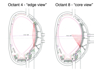
Figure 2: Line-of-sight coverage of the JET edge CXRS system (KS7), viewing Octant 4 and Octant 8 neutral beams.
