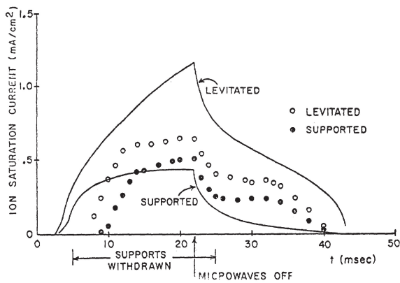
Fig. (3) Comparison of computer prediction (solid lines) and experimental measurement (dots) of ion saturation current time histories. Same parameters as for Fig. (2), rings supported and levitated.
