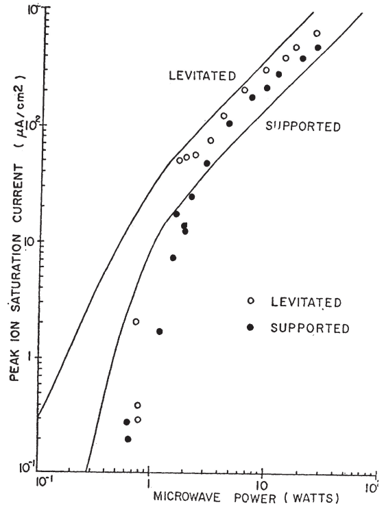
Fig. (4) Comparison of computer prediction (solid lines) and experimental measurement (dots) of peak ion saturation current for varying microwave power. Other parameters are the same as for Fig. (2), rings supported and levitated. (Log-log plot).
