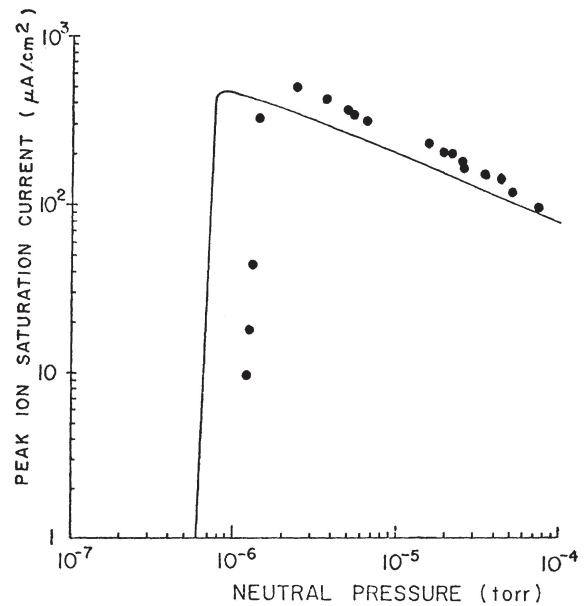
Fig. (5) Comparison of computer prediction (solid line) and experimental measurement (dots) of peak ion saturation current for varying neutral pressure. Other parameters are the same as for Fig. (2). (Log-log plot).
