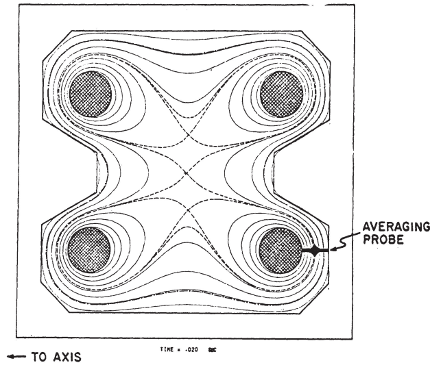
Fig. (1) Minor cross section of the Wisconsin Levitated Toroidal Octupole, showing lines of magnetic flux at 20 msec. after start of magnetic field pulse. Also shown is position of averaging probe. (Probe not to scale).
