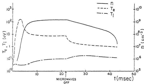
Fig. (2) Computer prediction of n , T_e , and T_i time histories. B_0 = 1 KG, p_{oi} = .125 \times 10^{-5} torr, P = 25 W, rings supported. (Semilog plot).
