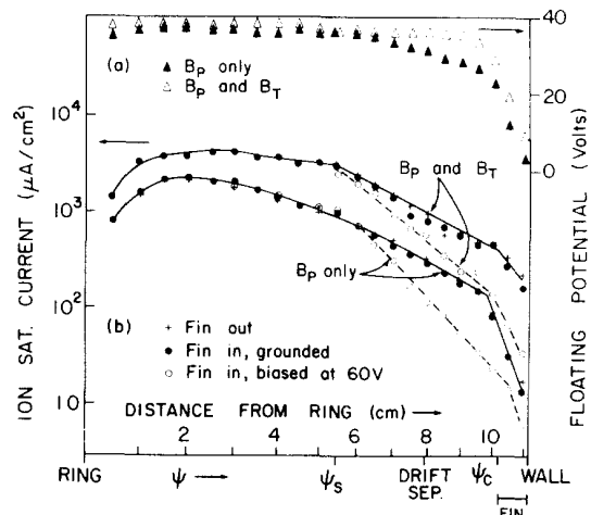
FIG. 4. Radial profiles of (a) floating potential and (b) ion saturation current, 15^\circ downstream from fin. V_r = 40 V. Location of drift separatrix is taken from Fig. 3(a).
