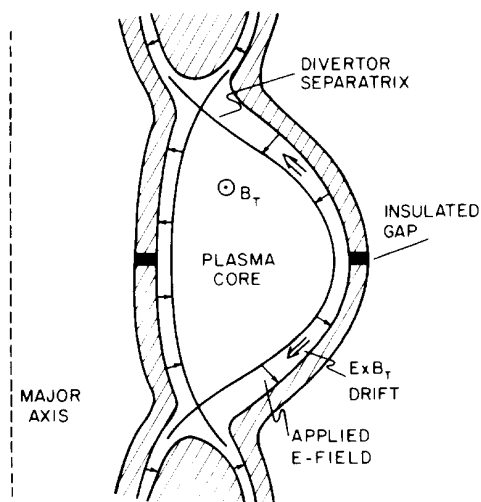
FIG. 1. Minor cross section of tokamak with double-poloidal-null divertor. Radial electric field (arrows) applied by biased wall segments results in \mathbf{E} \times \mathbf{B}_t drift (double arrows) toward pumping chamber.
