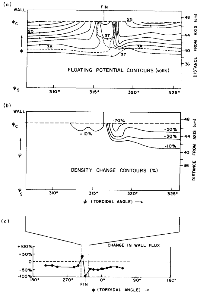
FIG. 3. Experimentally measured quantities plotted vs \phi (toroidal angle). V_r = 40 V, V_d = 60 V, B_p only. (a) and (b) are contour plots in \psi (poloidal flux function) and \phi . Distance from minor axis along midcylinder is also shown. (a) Floating potential contours at 2-V intervals. Arrowheads show direction of resulting E \times B drift. Dotted line (36.2 V contour) is drift separatrix. (b) Contours of relative change in density. (c) Relative change in wall flux. Vertical dotted lines show range in \phi of Figs. 3(a) and (b).
