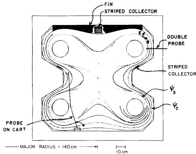
FIG. 2. Minor cross section (with poloidal flux lines) of Wisconsin levitated octupole, showing locations of retractable fin and diagnostics (not all at same toroidal position). \psi_s is octupole separatrix, \psi_c is last magnetohydrodynamically stable field line (minimum of \oint dl/B ).
