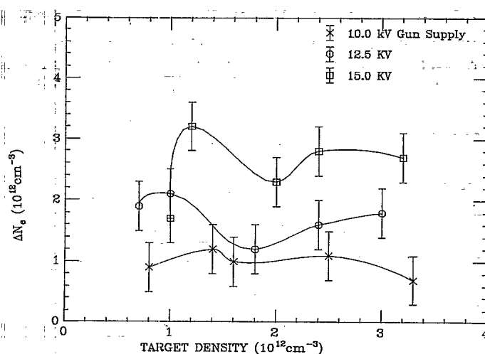
FIG. 5. The trapping of gun-injected plasma depends very little on line-averaged Tokapole II electron density (target density).
