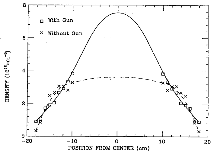
FIG. 3. Density profile found by use of Langmuir probe at edge and line-integrating interferometer.
