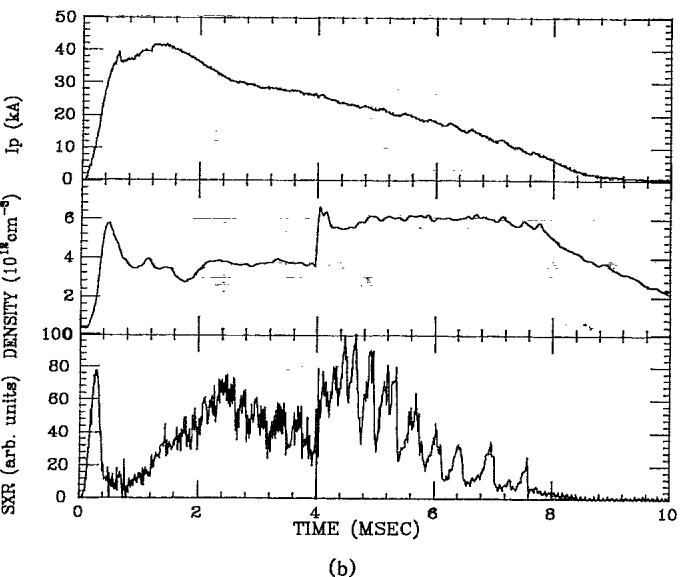
FIG. 2. Characteristics of Tokapole II discharge (a) without and (b) with gun refueling. Shown are the plasma current ( I_p ), line-averaged electron density ( N_e ), and central-chord soft x-ray emissivity (SXR).
