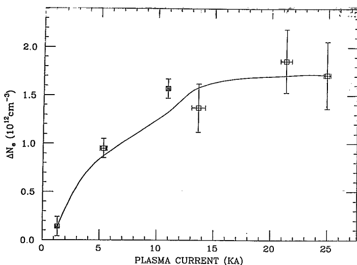
FIG. 4. Trapping efficiency ( \Delta N_e ) shows strong correlation with plasma current.
