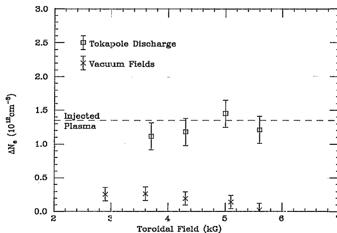
FIG. 6. Trapped density for tokamak discharge is greater than for corresponding vacuum-field case.
