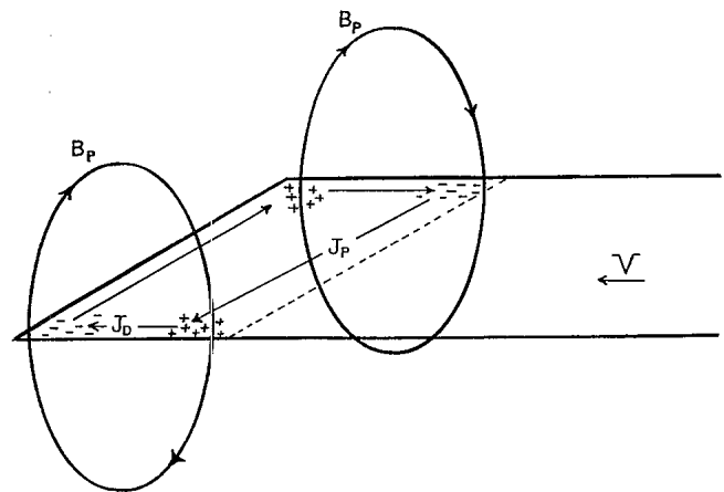
FIG. 1. Trapping mechanism for plasma injected into poloidal magnetic field. The polarization current ( J_p ) provides a \mathbf{J} \times \mathbf{B} force to plasma moving with velocity \mathbf{V} . The depolarization current ( J_D ), resulting from field reversal, drains charge buildup due to J_p and allows J_p to continue flowing until plasma is stopped.
