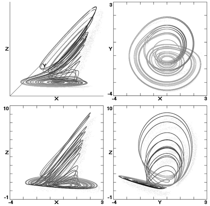
Fig. 1. Chaotic attractor from Eq. (4) with a = 2 and initial condition (x_0, y_0, z_0) = (0, 0, 2) .
