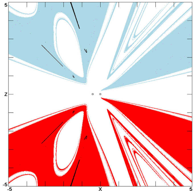
Fig. 7. Cross sections in the plane x = -y of the basins of attraction (red and blue, respectively, in the web version) for the two hidden strange attractors whose cross sections are shown in black for Model SL_3 . Two of the three unstable equilibria (shown as small open circles) lie outside both basins as does the third equilibrium (shown in Fig. 4), and all orbits that start in the vicinity of these equilibria are unbounded.
