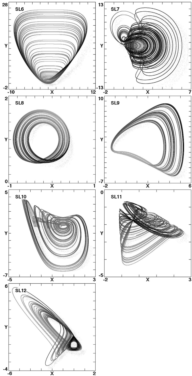
Fig. 5. State space diagram for the cases in Table 2 projected onto the xy -plane.
